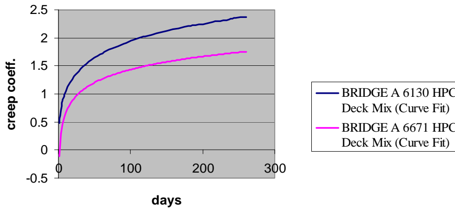
Figure 5.1 Creep Comparison Curve
