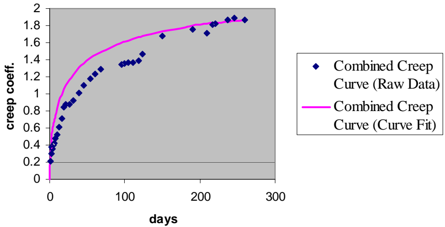
Figure 4.2 Combined Behaviors of Three Creep Specimens (Raw and Curve fit Data)
