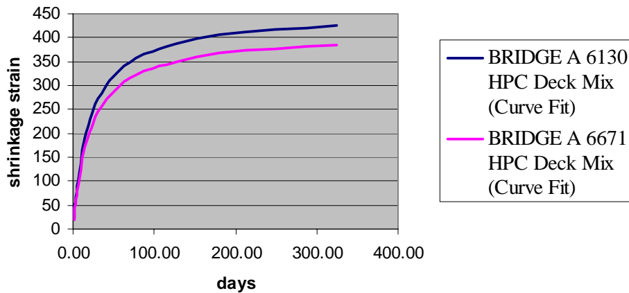
Figure 5.2 Shrinkage Comparison Curve
