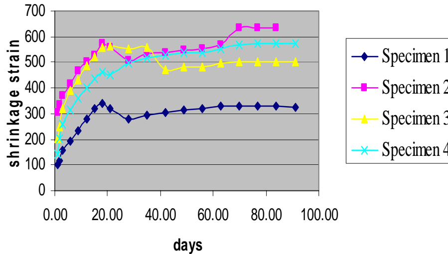
Figure 4.3 Individual Behaviors of 4 Shrinkage Specimens for Deck A6671(Raw Data)
