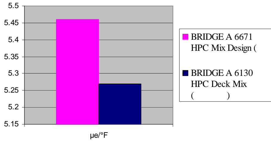
Figure 5.3 CTE Comparison Curve
