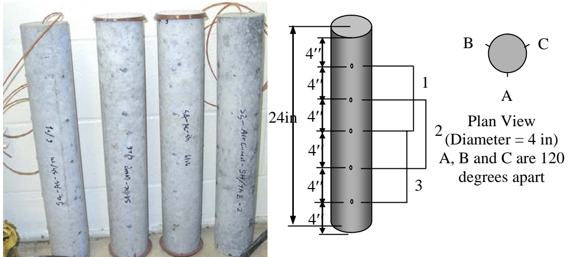
Figure 3.1 C/S/T Specimens and DEMEC Points Arrangement
