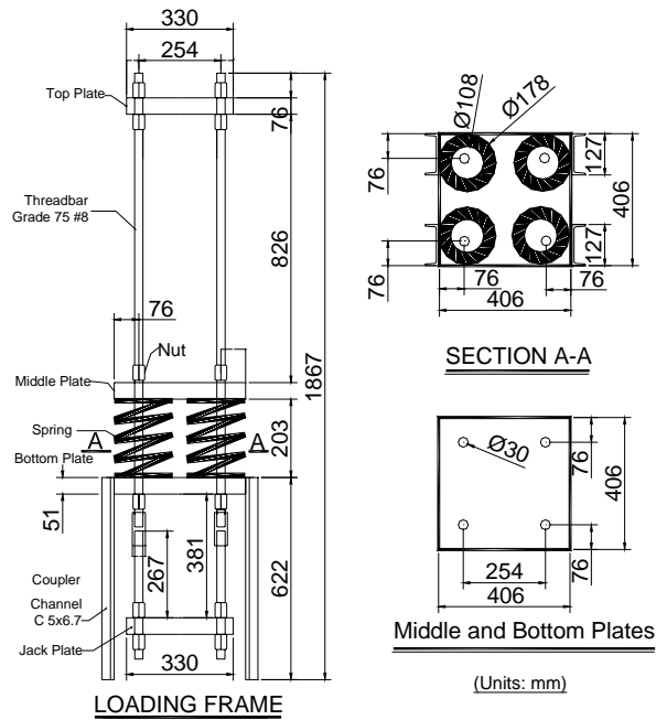
Figure 3.2 Creep Loading Frame and Specimens
