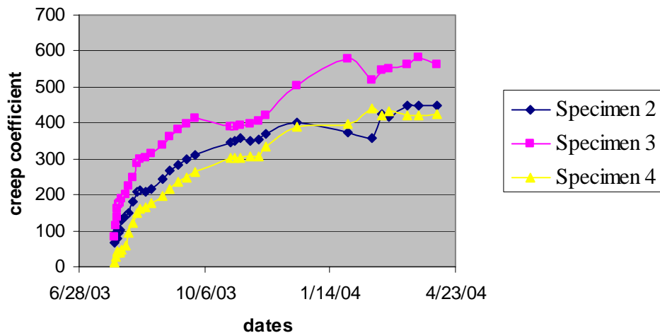
Figure 4.1 Individual Behaviors of Three Creep Specimens (Raw Data)
