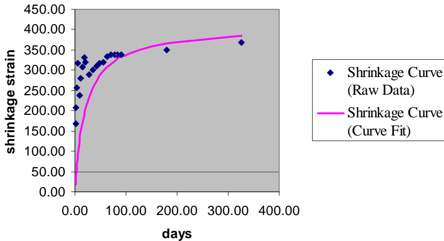
Figure 4.4 Combined Behaviors of Four Shrinkage Specimens (Raw Data and Curve Fit)
