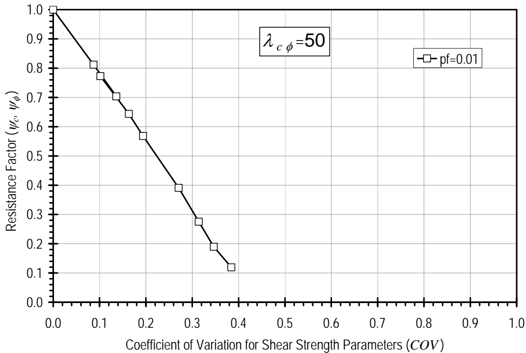
Figure 5.7 Resistance factor relations for c ( \psi_c ) and \tan \phi ( \psi_{\tan \phi} ) for conditions where \lambda_{c\phi} = 50 and p_f = 0.01 .
