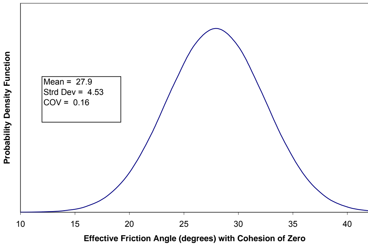
Figure A.7. Histogram and probability density function for effective friction angle, with zero cohesion, of low plasticity clay (CL).
