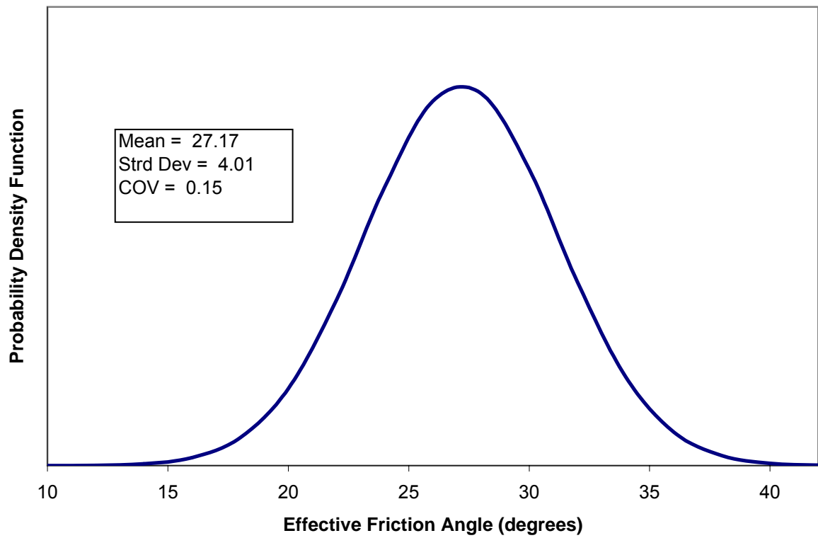
Figure D.5. Histogram and probability density function for effective friction angle for silty clay (CL-ML).
