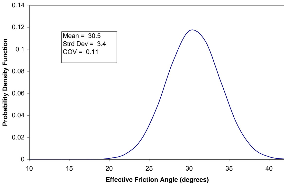
Figure C.5. Histogram and probability density function for effective friction angle of silt (ML).
