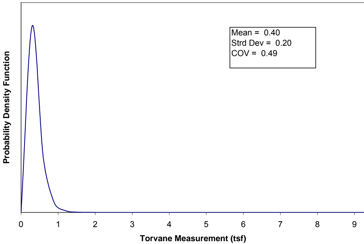
Figure A.2. Histogram and probability density function for torvane measurements for low plasticity clay (CL).
