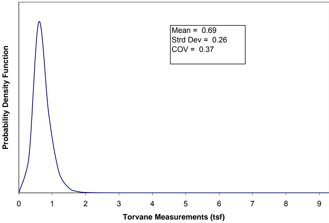
Figure B.2. Histogram and probability density function for torvane measurements for high plasticity clay (CH).
