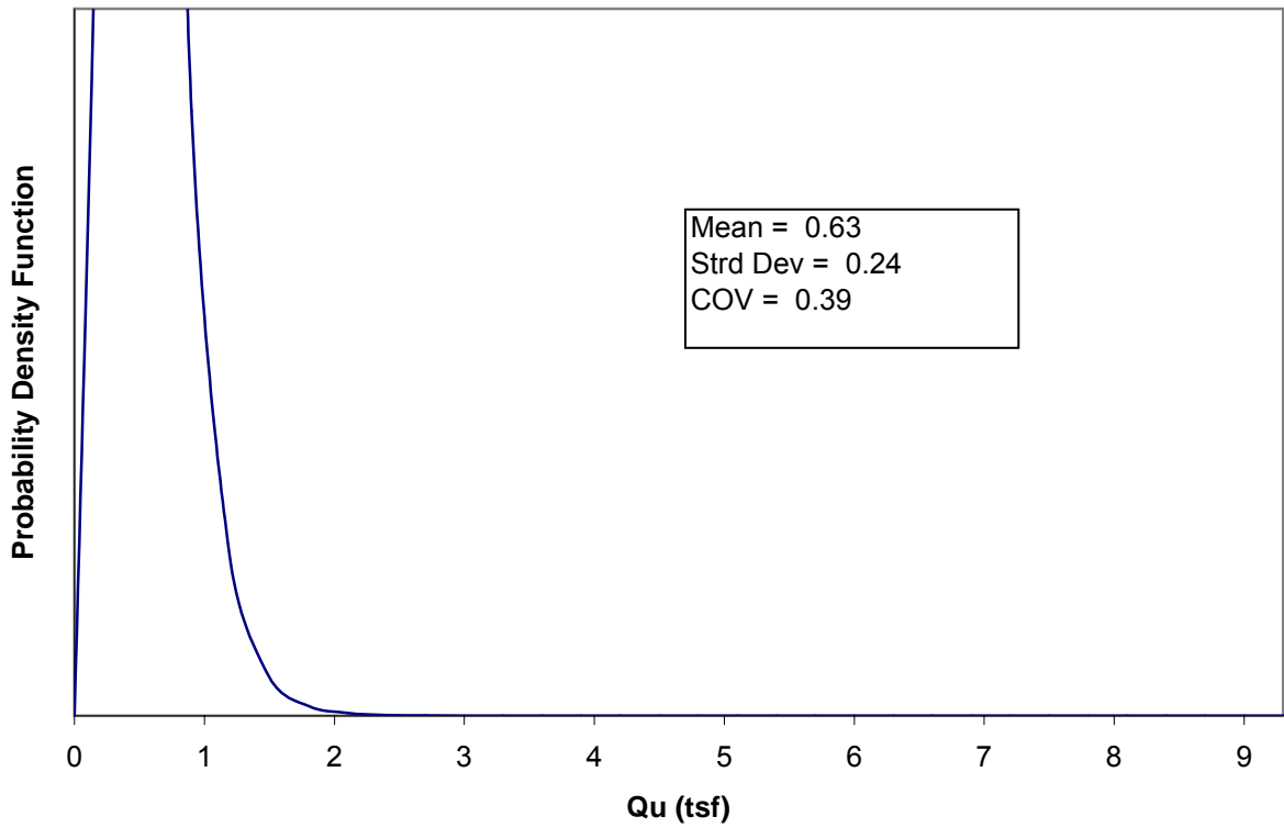
Figure C.3. Histogram and probability density function for unconfined compression tests for silt (ML).
