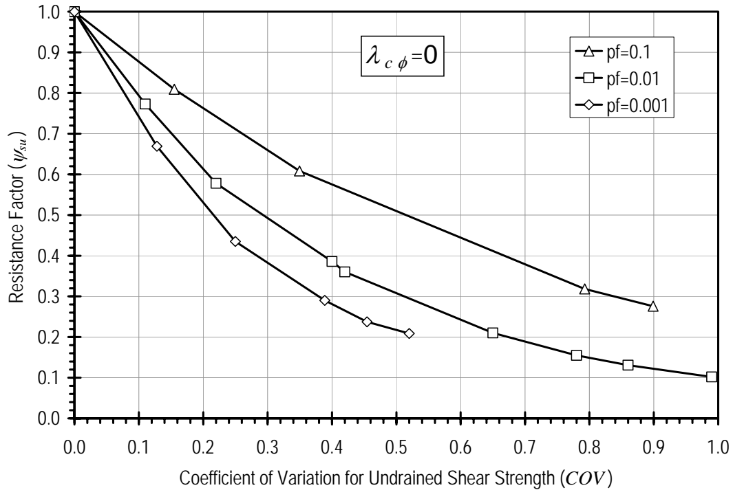
Figure 5.9 Resistance factor relations for undrained shear strength ( \psi_{su} ) for conditions where \lambda_{c\phi} = 0 and p_f = 0.1, 0.01, \text{ and } 0.001 .
