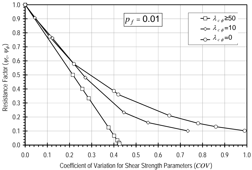
Figure 5.12 Recommended form of "resistance factor chart" for design of earth slopes for probability of failure, p_f=0.01 (1 in 100).
