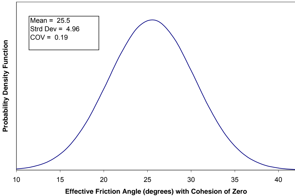
Figure B.6. Histogram and probability density function for effective friction angle of high plasticity clay (CH).
