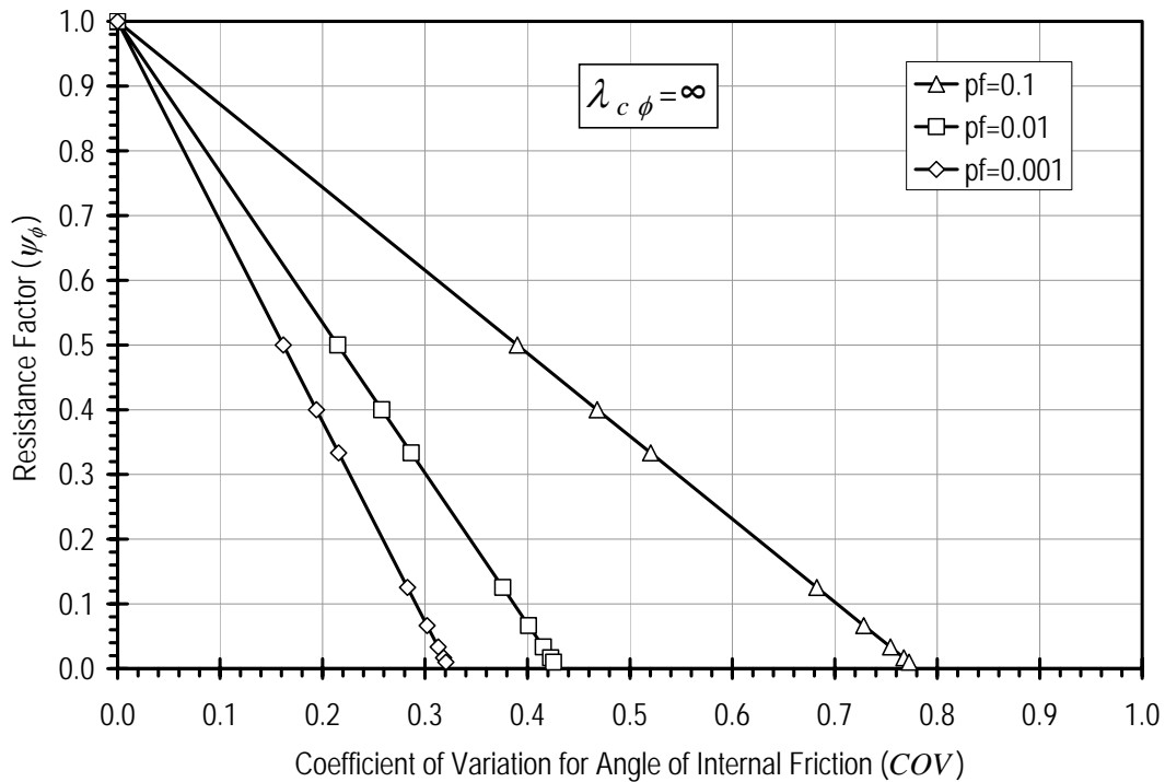
Figure 5.6. Resistance factors relations for \tan \phi ( \psi_{\tan \phi} ) for conditions where \lambda_{c\phi} = \infty and p_f = 0.1, 0.01, \text{ and } 0.001 .
