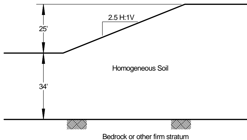
Figure 5.4. General slope geometry utilized for calibration of load and resistance factors in this project.
