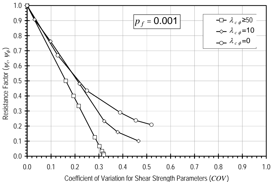
Figure 5.13 Recommended form of “resistance factor chart” for design of earth slopes for probability of failure, p_f=0.001 (1 in 1000).
