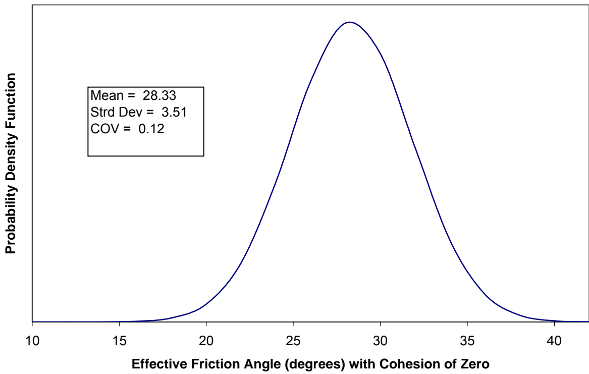
Figure D.7. Histogram and probability density function for effective friction angle, with zero cohesion, of silty clay (CL-ML).
