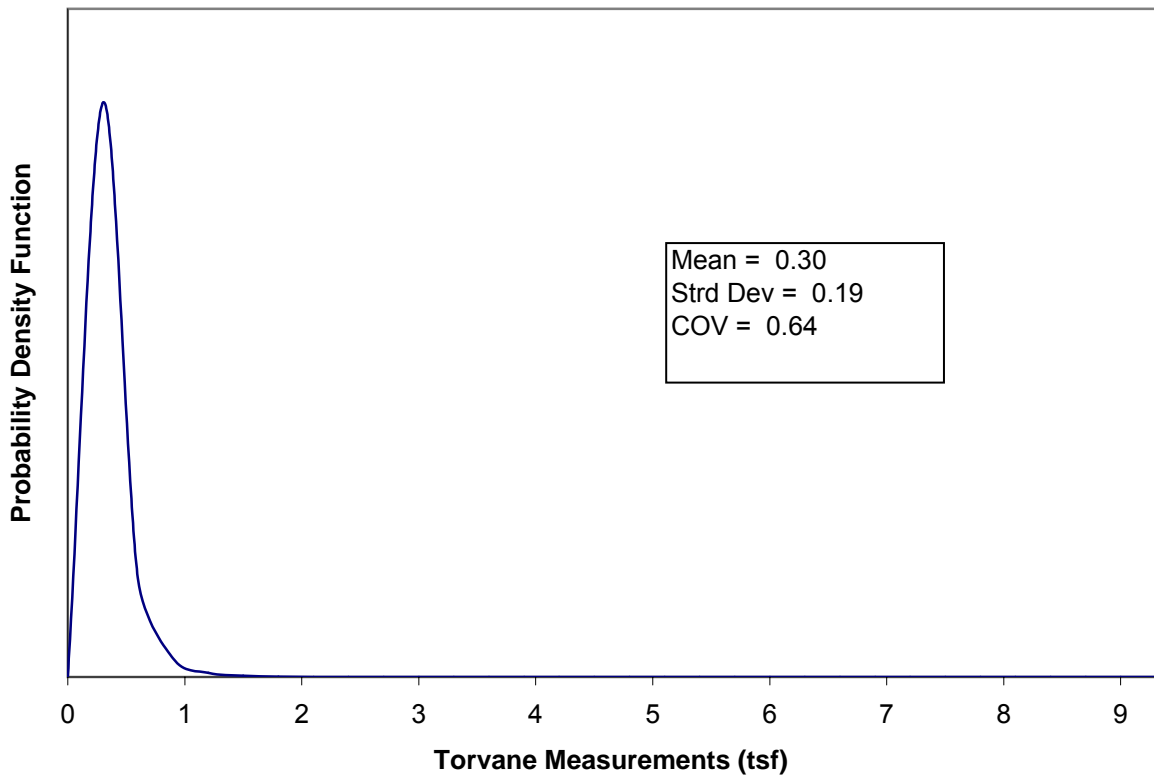
Figure C.2. Histogram and probability density function for torvane measurements for silt (ML).
