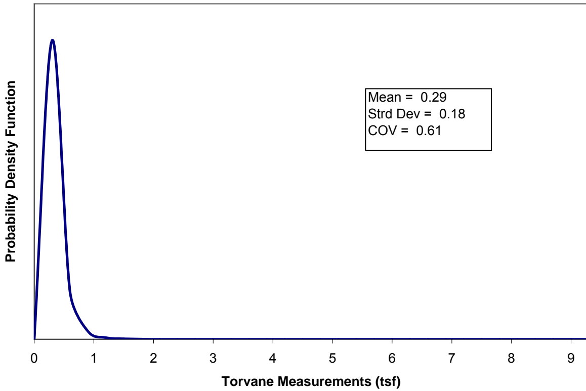
Figure D.2. Histogram and probability density function for torvane measurements for silty clay (CL-ML).
