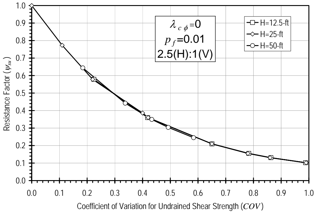
Figure 5.11 Comparison of resistance factor relations for slopes with different slope heights for \lambda_{c\phi}=0 and p_f=0.01 .
