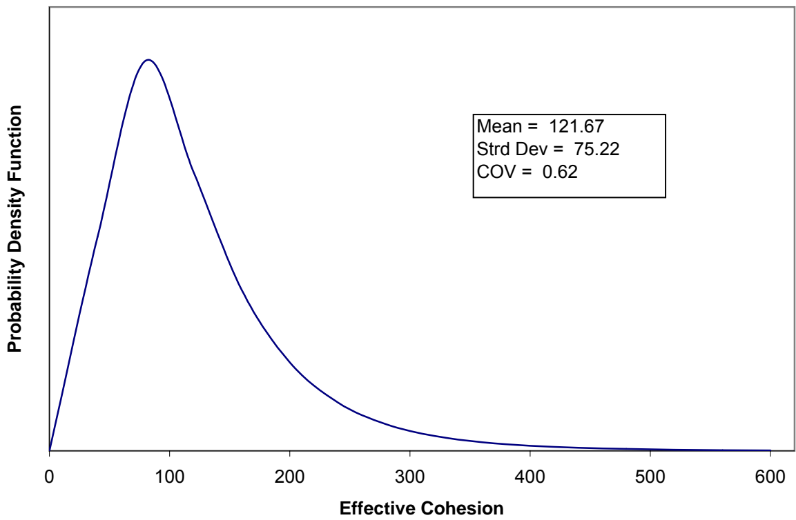
Figure D.6. Histogram and probability density function for effective cohesion of silty clay (CL-ML).
