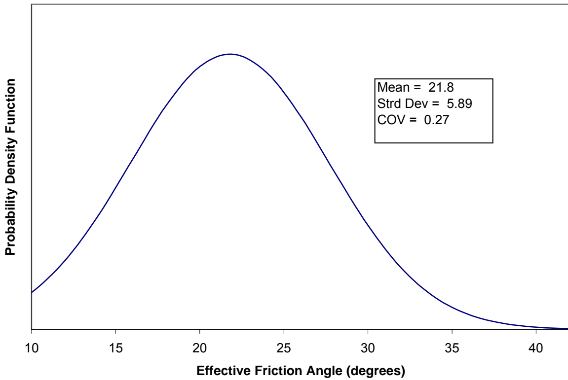
Figure B.4. Histogram and probability density function for effective friction angle of high plasticity clay (CH).
