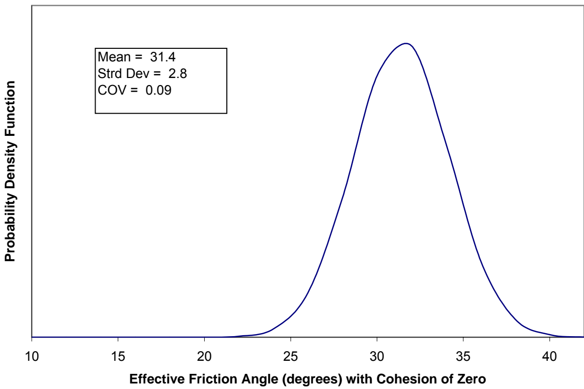
Figure C.7. Histogram and probability density function for effective friction angle, with zero cohesion, of silt (ML).
