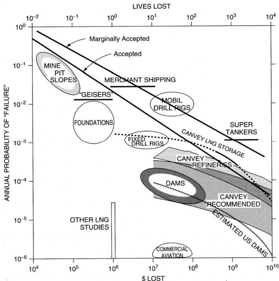
Figure 5.5. Diagram illustrating relationship between annual probability of failure and risk (expressed in terms of $ lost and lives lost) for common civil facilities (from Baecher and Christian, 2003).
