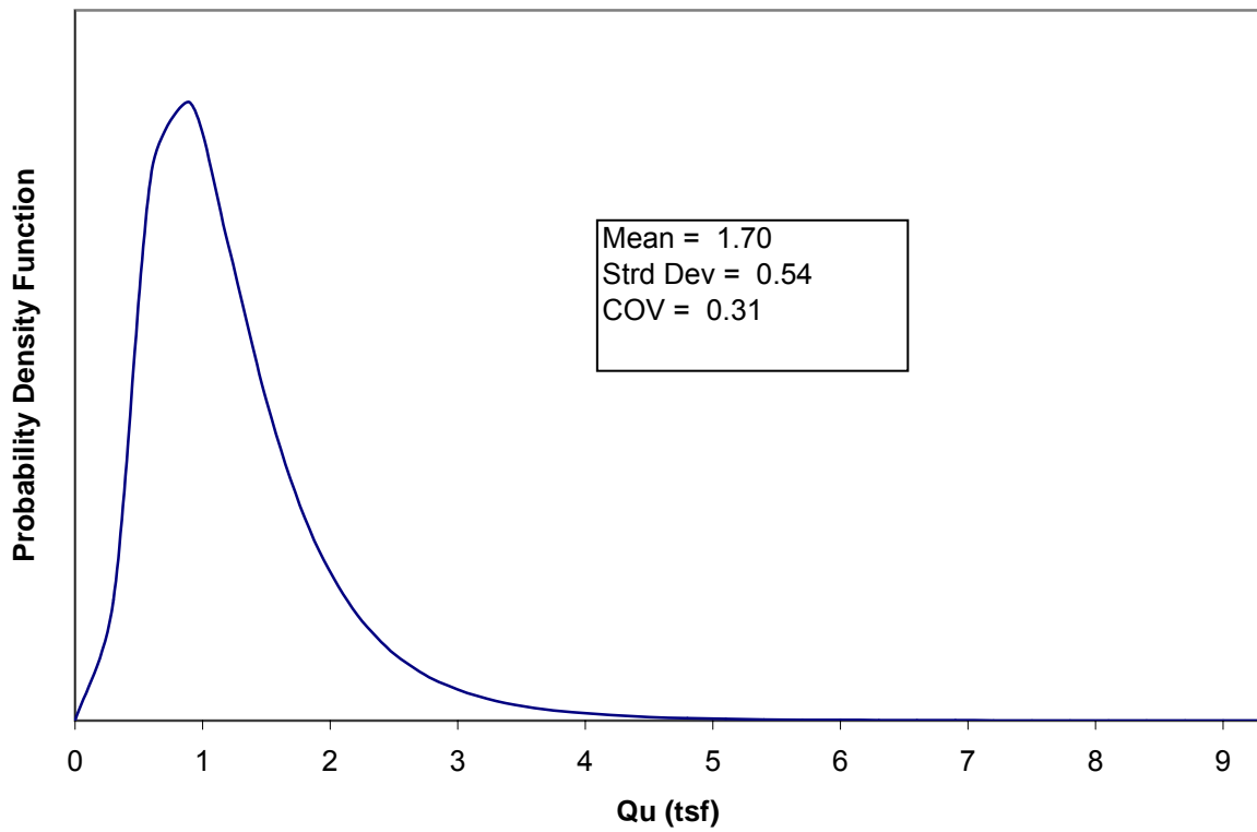
Figure B.3. Histogram and probability density function for unconfined compression tests for high plasticity clay (CH).
