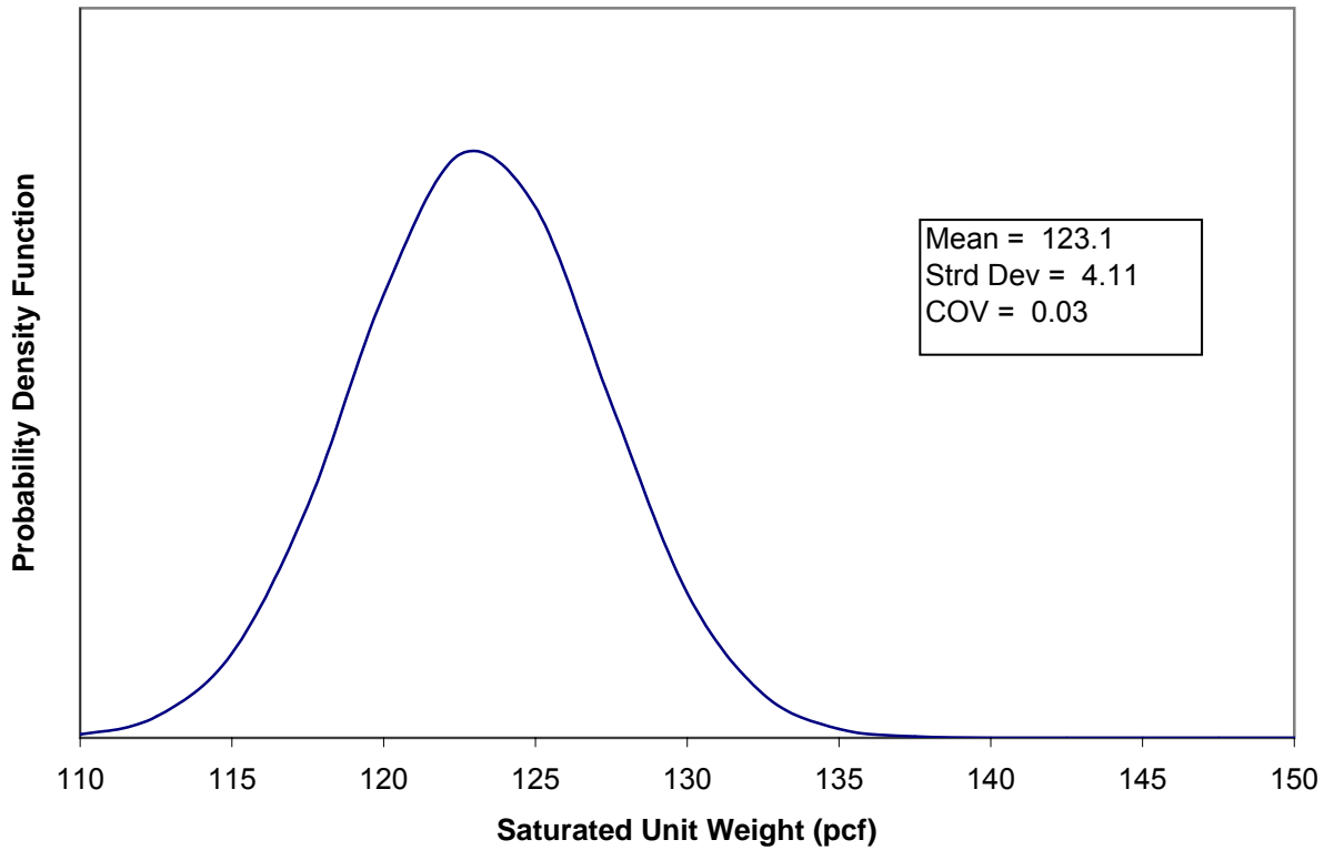
Figure A.4. Histogram and probability density function for saturated unit weight of low plasticity clay (CL).
