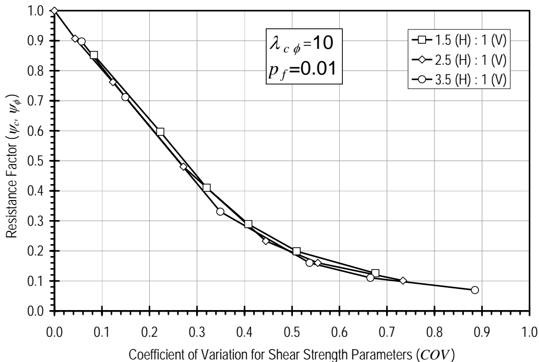
Figure 5.10 Comparison of resistance factor relations for slopes with different slope angles for \lambda_{c\phi}=10 and p_f=0.01 .
