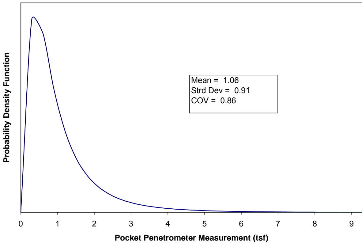
Figure A.1. Histogram and probability density function for pocket penetrometer measurements for low plasticity clay (CL).
