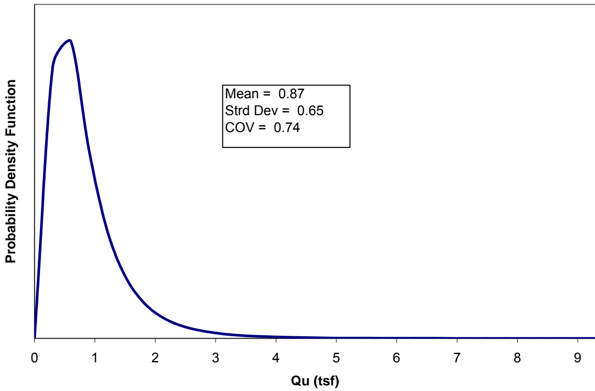
Figure D.3. Histogram and probability density function for unconfined compression tests for silty clay (CL-ML).
