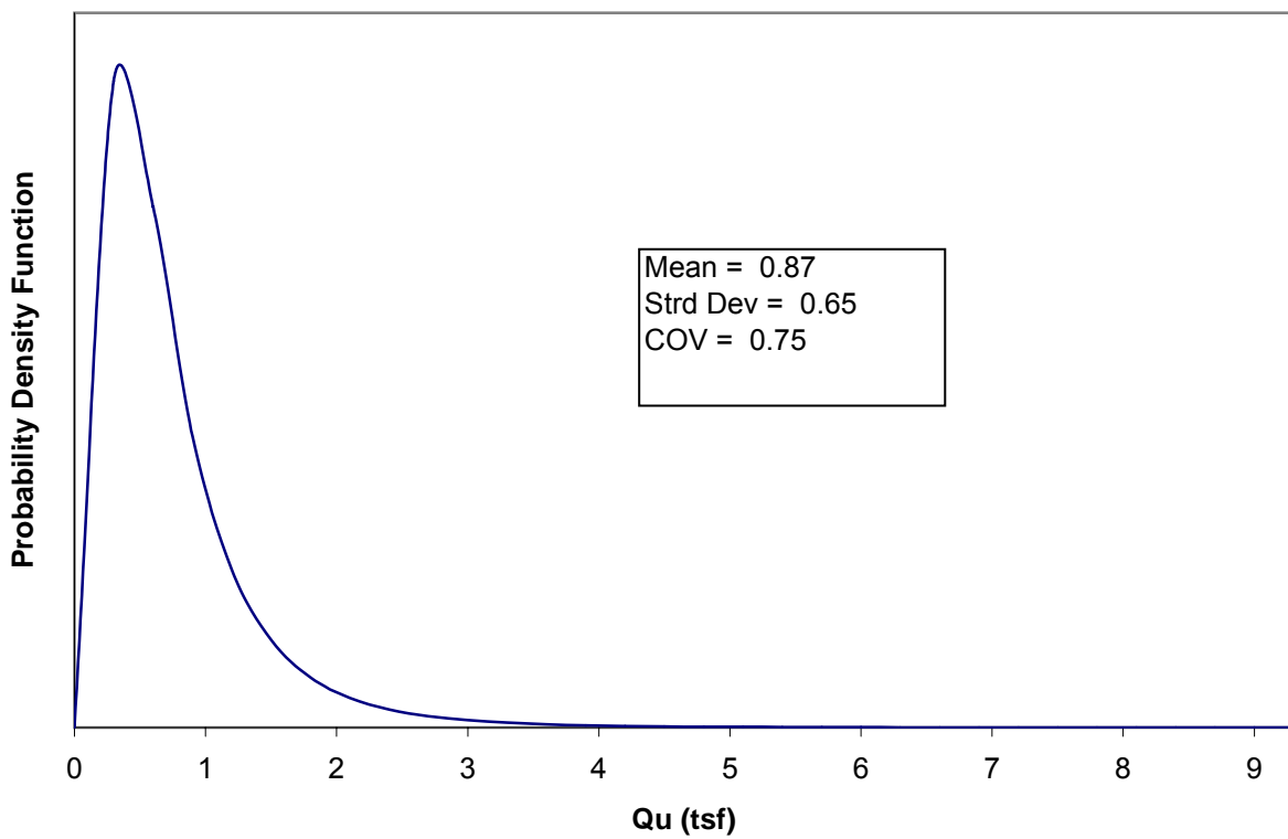
Figure A.3. Histogram and probability density function for unconfined compression tests for low plasticity clay (CL).
