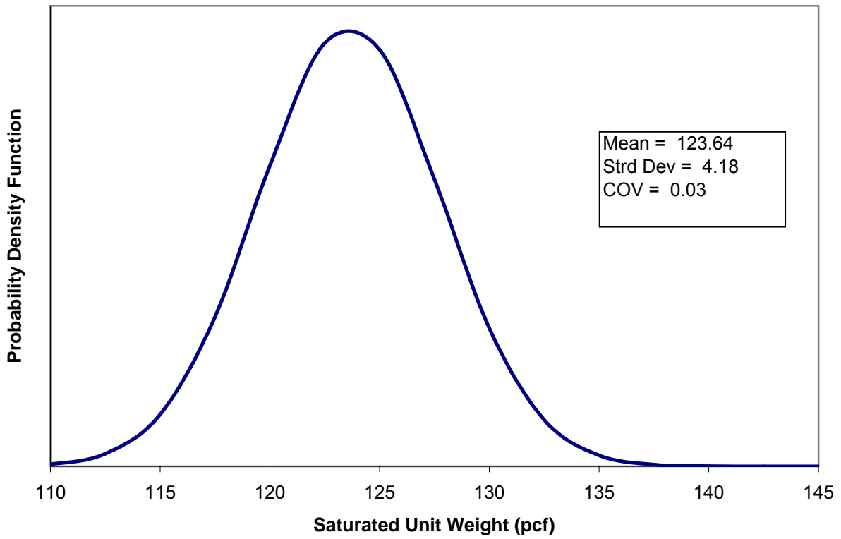
Figure D.4. Histogram and probability density function for saturated unit weight of silty clay (CL-ML).
