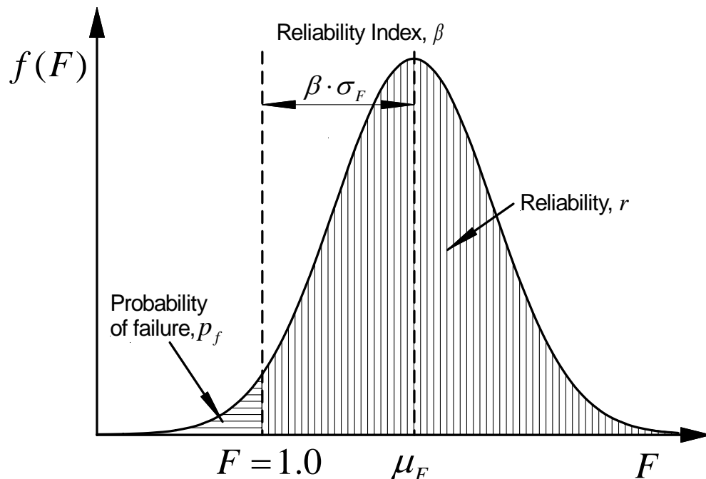
Figure 5.3. Sample distribution of factor of safety illustrating commonly used measures of safety for earth slopes.
