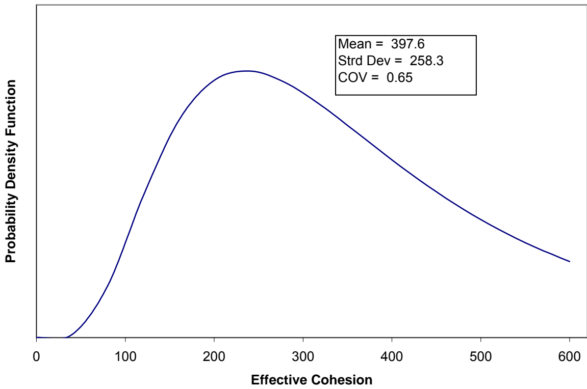
Figure B.5. Histogram and probability density function for effective cohesion of high plasticity clay (CH).
