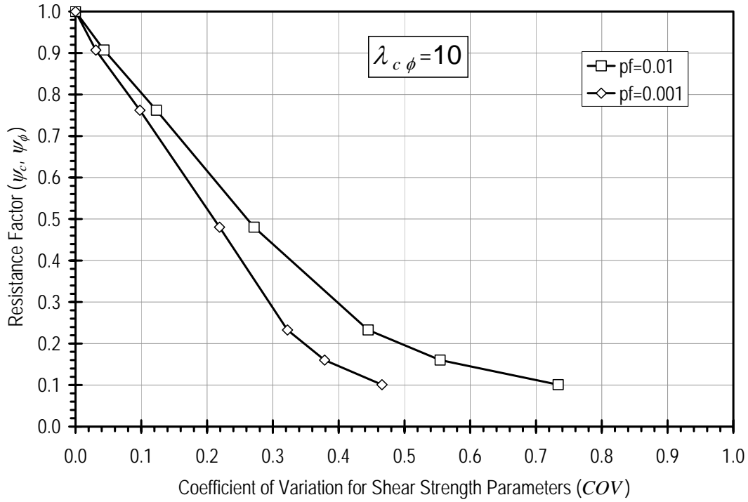
Figure 5.8 Resistance factor relations for c ( \psi_c ) and \tan \phi ( \psi_{\tan\phi} ) for conditions where \lambda_{c\phi} = 10 and p_f = 0.01 and 0.001 .
