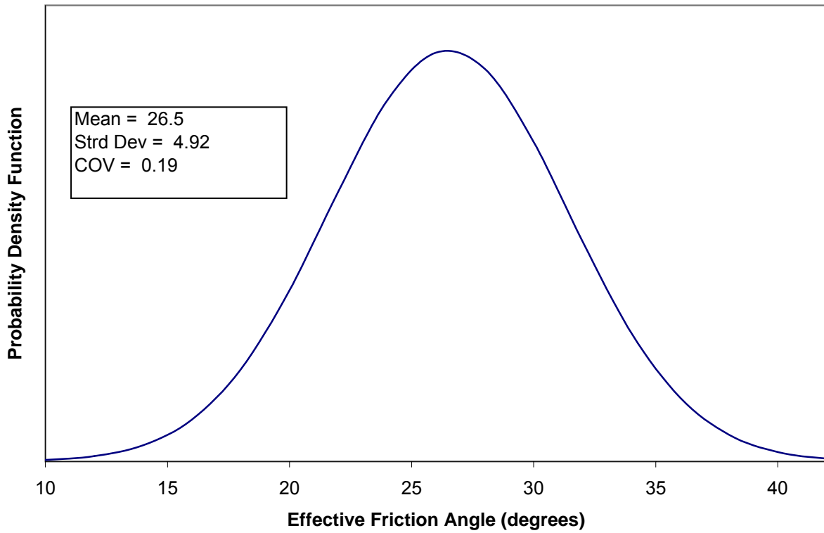
Figure A.5. Histogram and probability density function for effective friction angle of low plasticity clay (CL).
