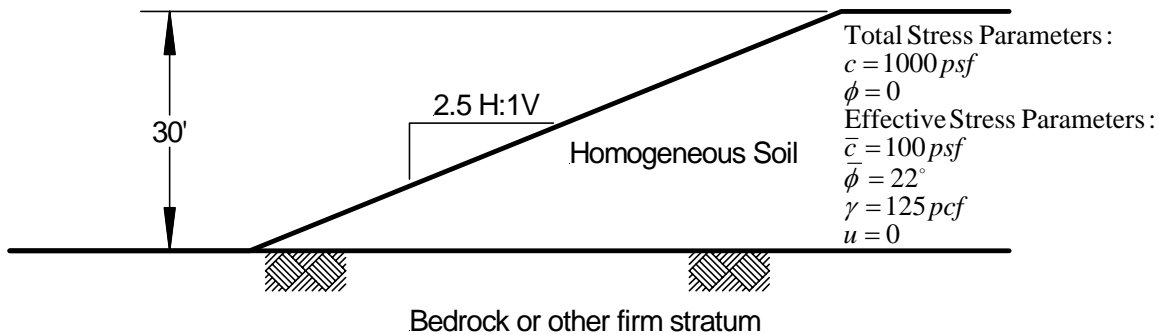
Figure 4.1 Slope conditions used for example problem.
