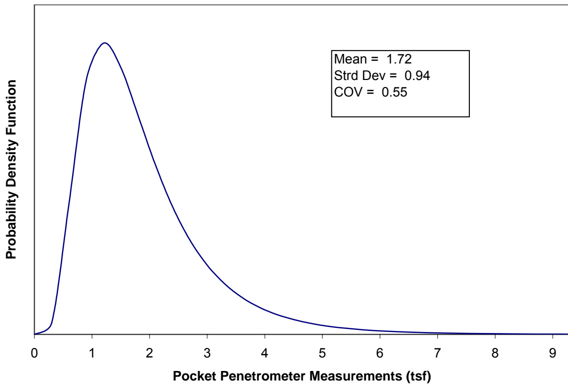
Figure B.1. Histogram and probability density function for pocket penetrometer measurements for high plasticity clay (CH).
