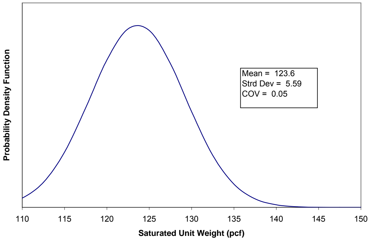
Figure C.4. Histogram and probability density function for saturated unit weight of silt (ML).
