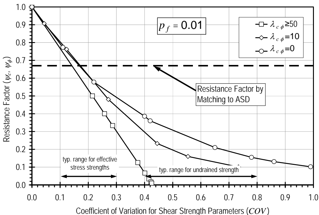
Figure 7.1 Comparison of resistance factor relations determined from probabilistic calibrations with relation established by matching to ASD for target F=1.5 .
