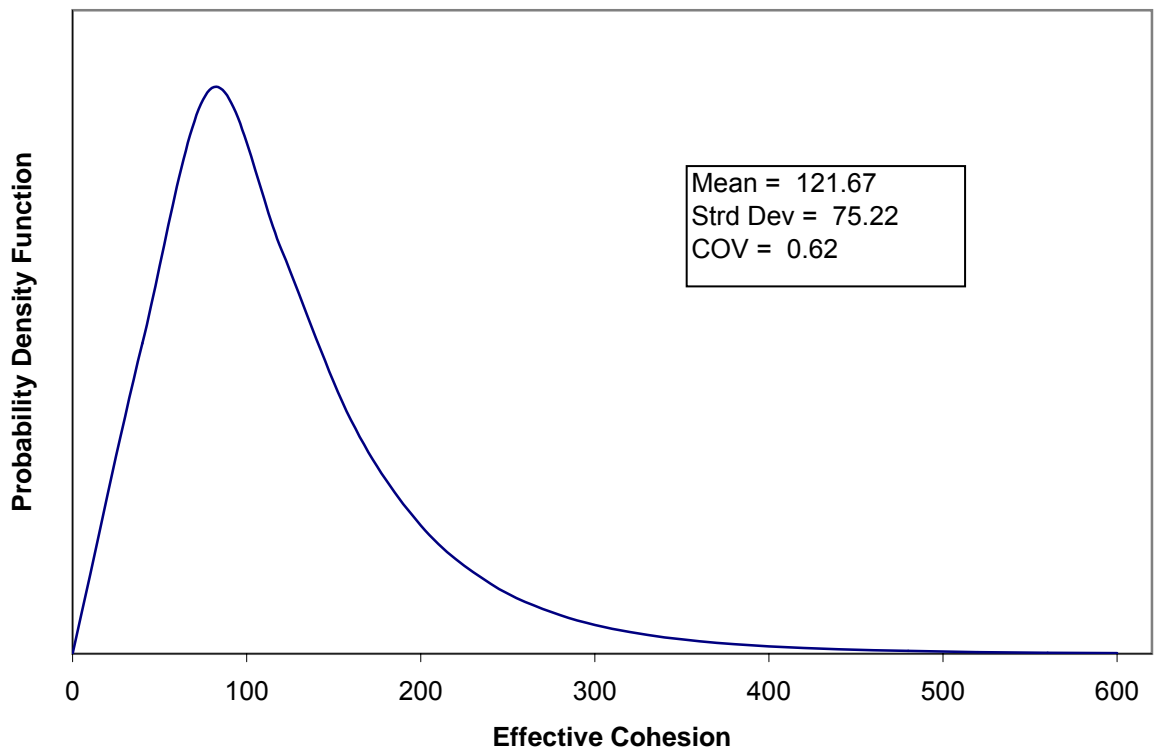
Figure D.6. Histogram and probability density function for effective cohesion of silty clay (CL-ML).
