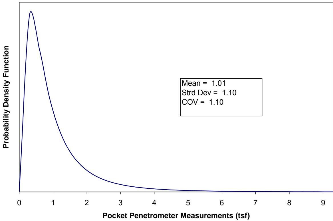
Figure C.1. Histogram and probability density function for pocket penetrometer measurements for silt (ML).
