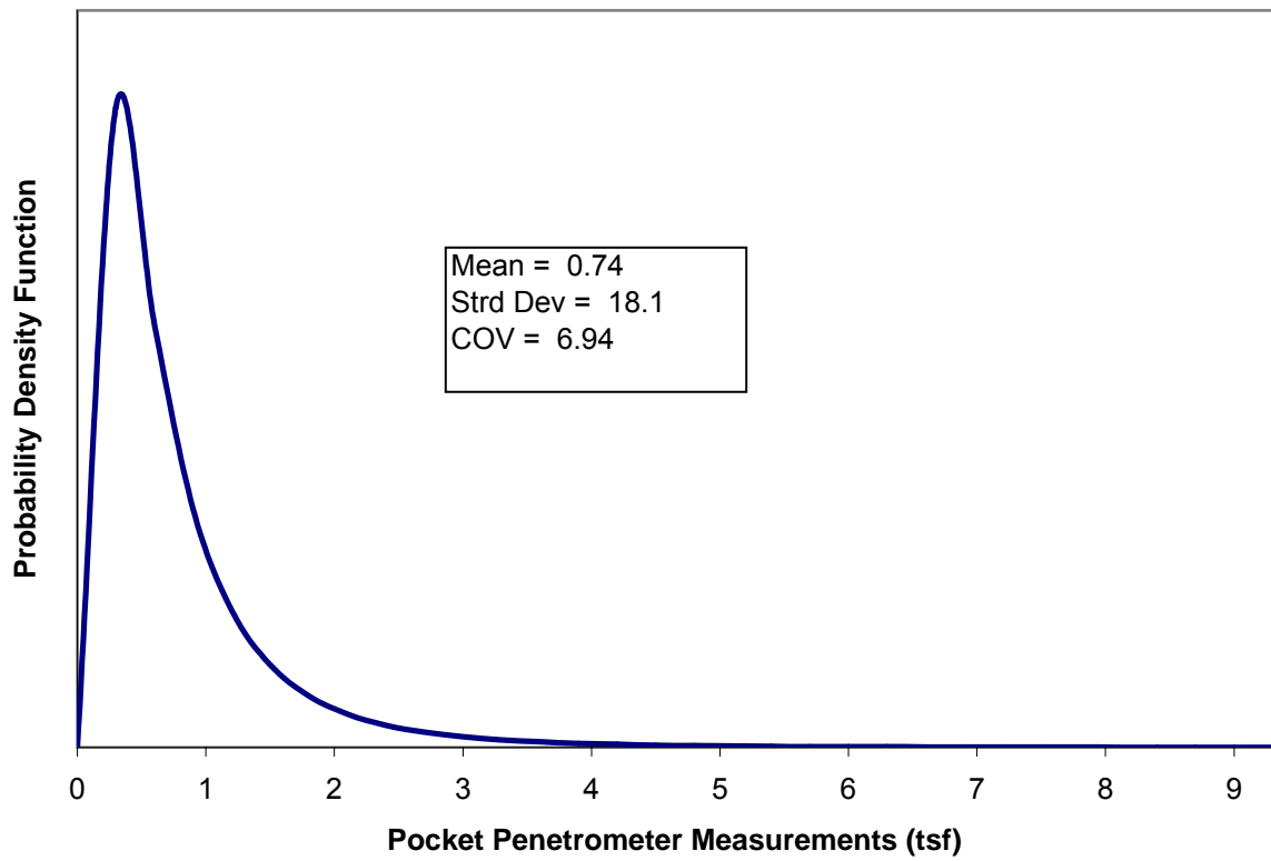
Figure D.1. Histogram and probability density function for pocket penetrometer measurements for silty clay (CL-ML).
