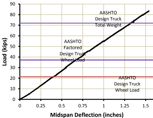
Load-Deflection Plot during Full Scale Test
